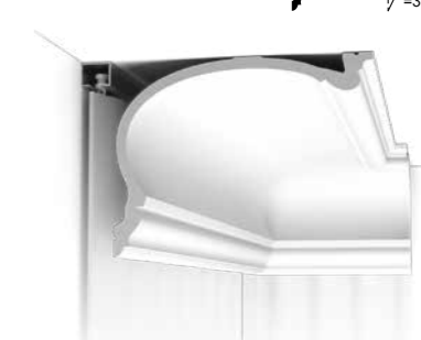
C343 HERITAGE CURTAIN PROFILE Purotouch® 200 x 19 x 25 cm
