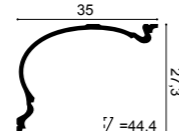
C344 HERITAGE Purotouch® 200 x 27,3 x 35 cm
