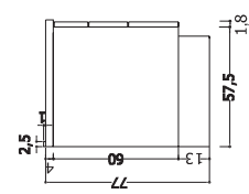
BASI H 73 BASE UNITS H 73
