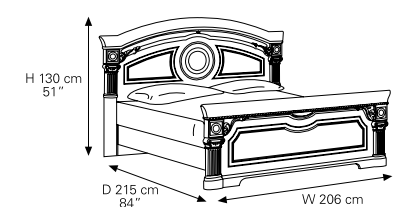
Aida bed KS cm 180 x 200/203 (mattress size) Also available cm 210 or cm 215 side rails Vol. 0,34 mc - Box 3 - Kg 72,50 099LET.02PI
