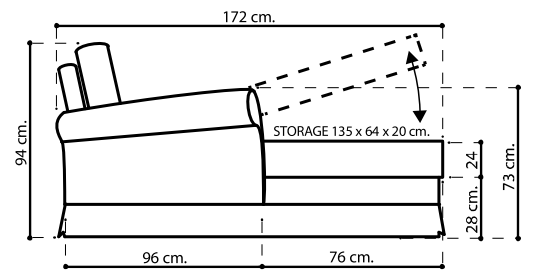
STORAGE – SIDE VIEW
