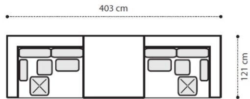
PAG.4 PIUMA Jsx + Jdx + Pouff121 + 2A + 2B + 2C note: Cuschions A, B, F in cat. B 403 x 121 x H. 63 cm
