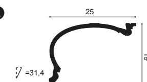
C343 HERITAGE A 200 x 19 x 25 cm Purotouch ®
