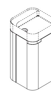
Free standing units Mobili freestanding W 45 X D 45 X H 88,5 cm
