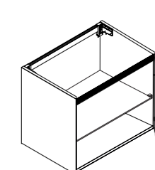
Wall mounted vanity unit with 1 door Base portlavabo sospesa con 1 anta W 60 cm D 38/46/51,5 cm
