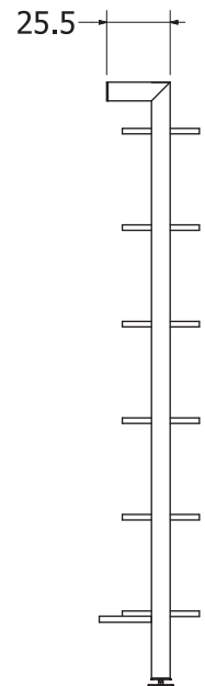
Vista laterale Side view
