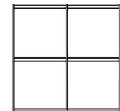
2/D SLIDING WARDROBE PJMN0020 With 2 doors, 2 shelves and 4 hanging rods inch W 90" D 26" H 94" cm L 228,7 P 65,5 H 239,1 Crts 9 kg 415 m 3 0,56
