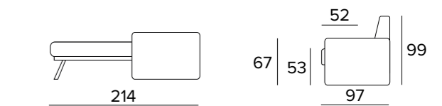
MATERASSO / MATELAS / MATTRESS CM 160x195 / H 21
