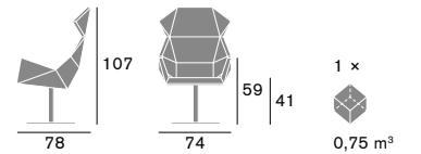
Prisma 1673 PO B01G Dimensioni / Sizes
